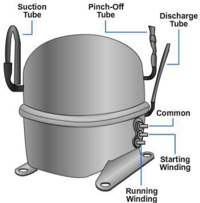
Figure 12-16 – Hermetic compressor.
