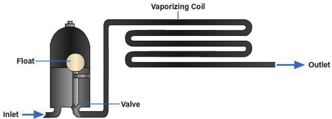
Figure 12-23 – Low-side float expansion valve.
