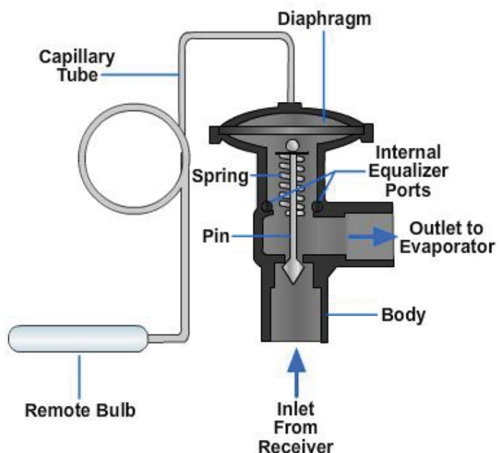
Figure 12-21 - Thermostatic expansion
