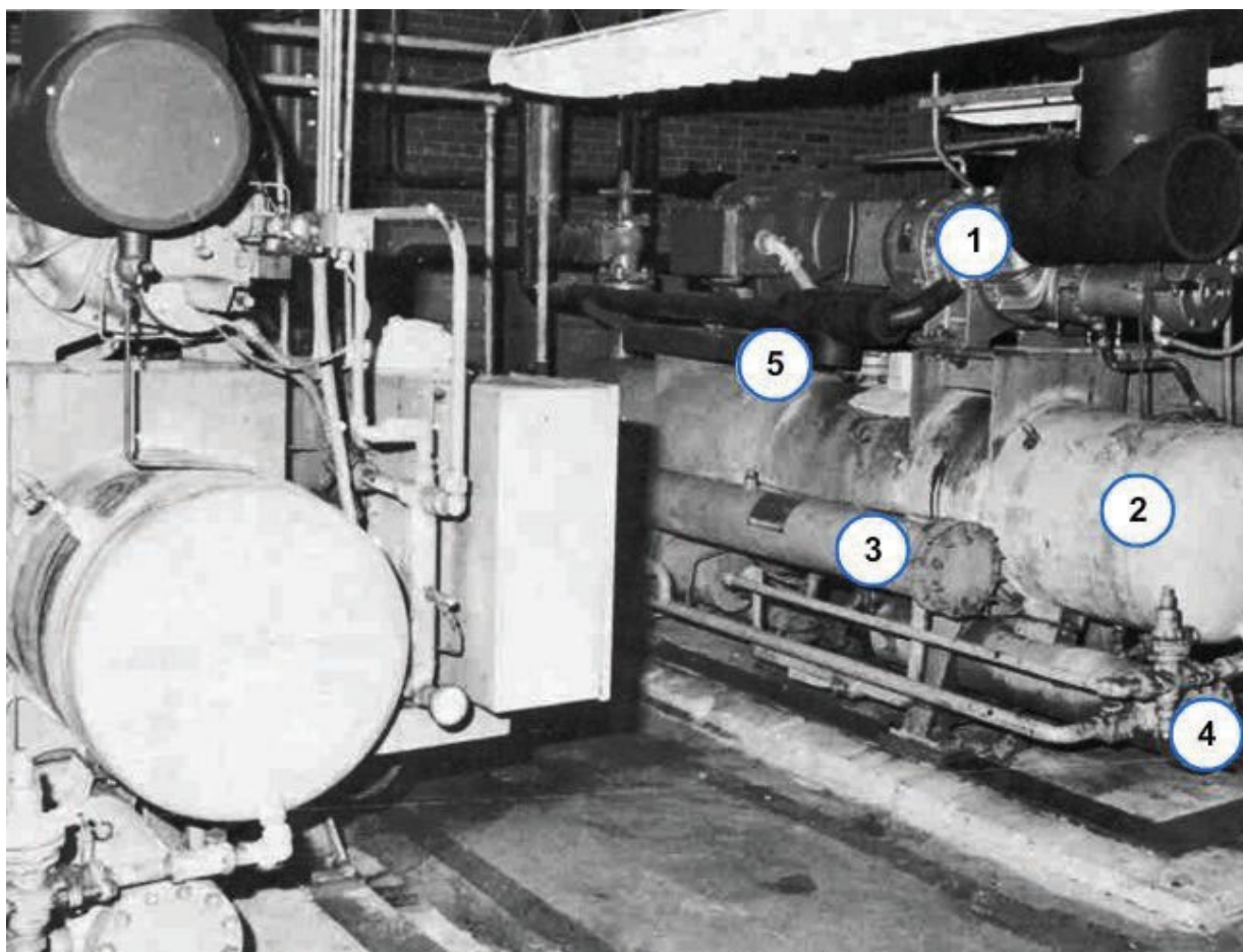
Figure 12-45 – Low-temperature screw or helix compressor system. (1) Compressor; (2) Oil separator and reservoir; (3) Oil cooler; (4) Oil filters; (5) Hot gas discharge line.
