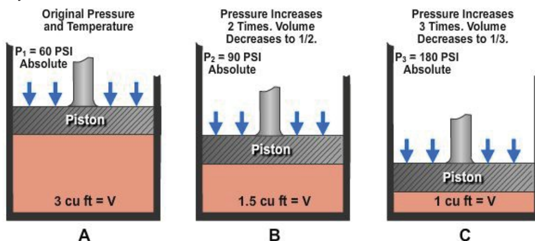
Figure 12-5 – Pressure-volume relationship.
