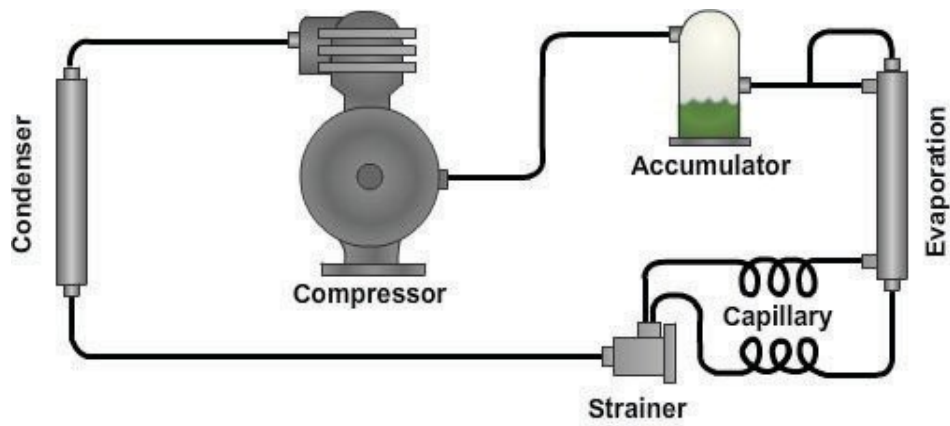
Figure 12-31 –Accumulator location.
