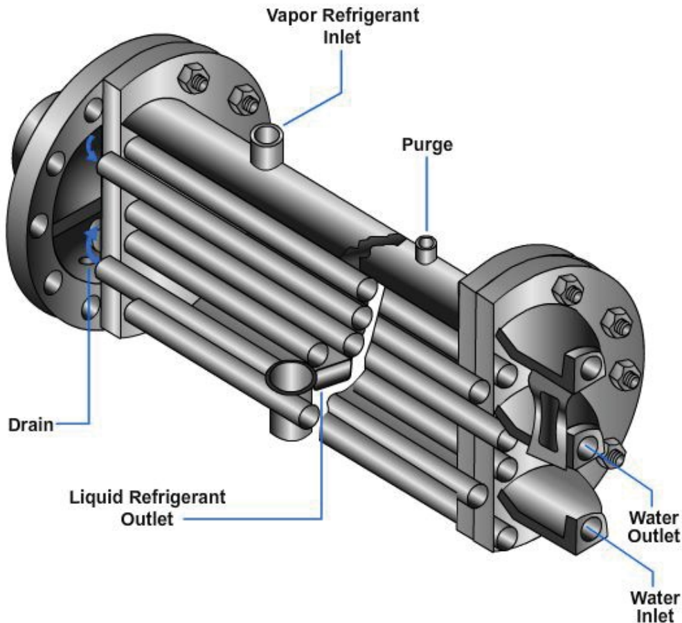
Figure 12-19 –Water-cooled condenser.
